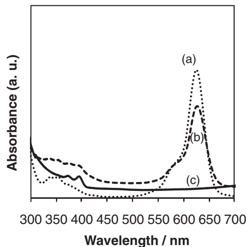
Figure 2. Absorption spectra of (a) BODIPY dye 1 ( 1.0 \times 10^{-5} M THF solution), and dye 1 -containing PHEMA–silica hybrids prepared under (b) microwave irradiation and (c) conventional heating. The feed ratio of HEMA/MeTMOS was 1/2. The molar ratio of HEMA/ 1 was 10000/1.
