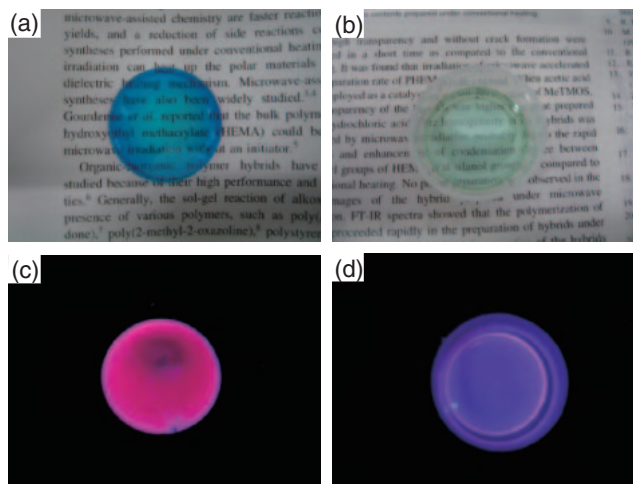
Figure 1. Photographs of BODIPY dye 1 -containing PHEMA–silica hybrids prepared under (a, c) microwave irradiation and (b, d) conventional heating, (a, b) appearance, (c, d) under UV irradiation. The molar ratio of HEMA/ 1 was 20000/1.
