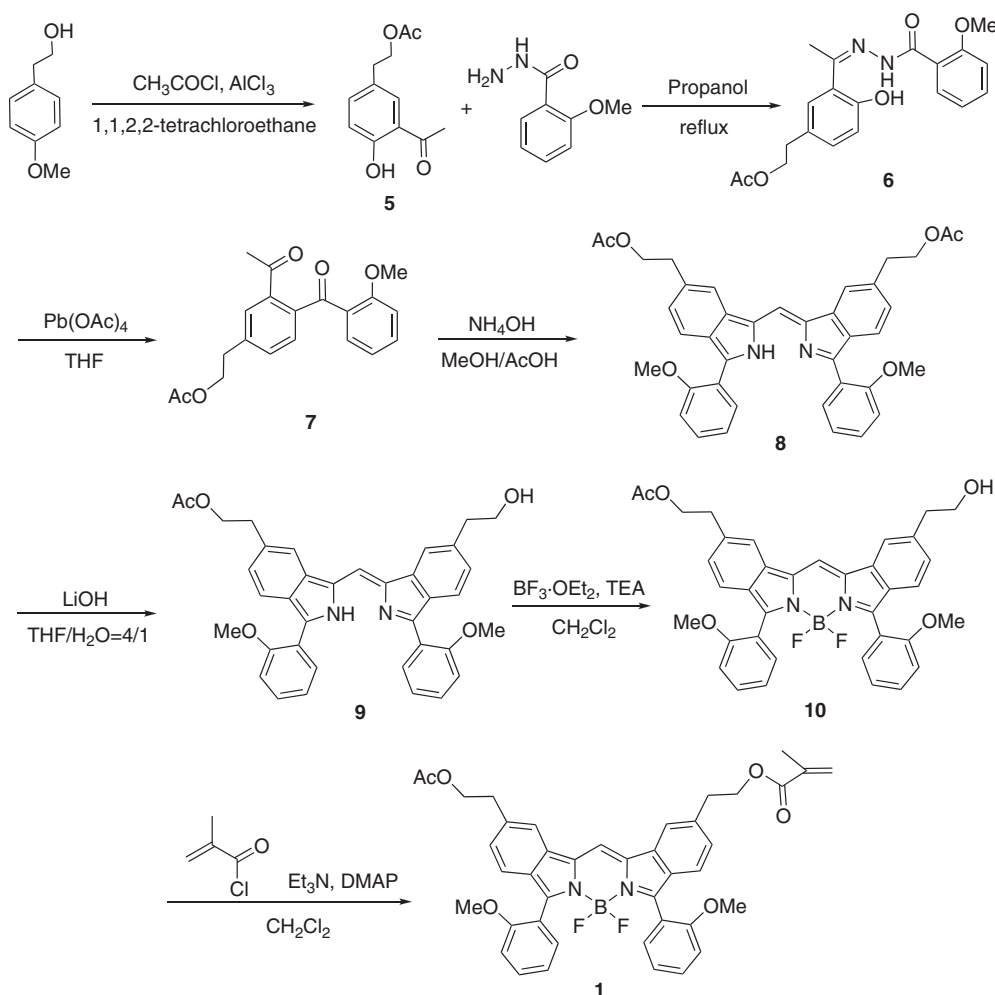
Scheme 2. Synthesis of methacrylate-tethered red light-emitting BODIPY dye 1 .
