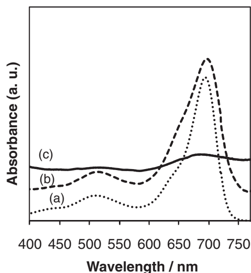
Figure 4. Absorption spectra of (a) BODIPY dye 2 ( 1.0 \times 10^{-5} M THF solution), and dye 2-containing PHEMA-silica hybrids prepared under (b) microwave irradiation and (c) conventional heating. The feed ratio of HEMA/MeTMOS was 1/2. The molar ratio of HEMA/2 was 10000/1.
