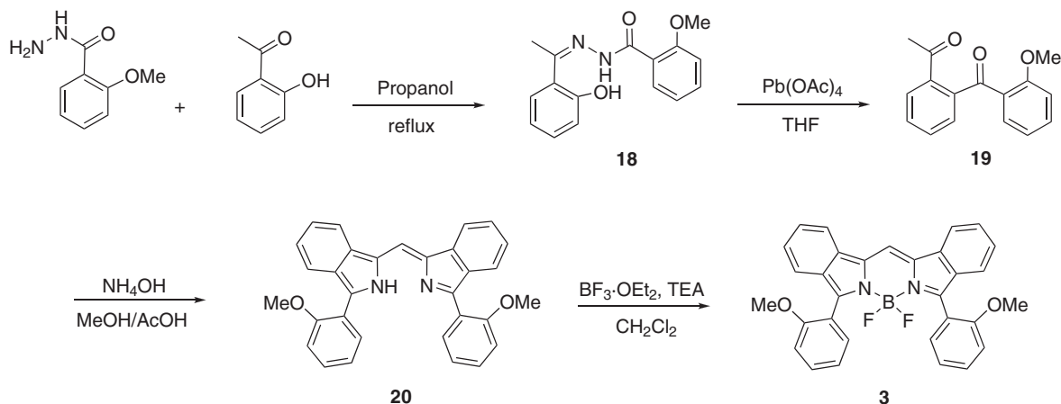
Scheme 4. Synthesis of boron di(iso)indomethene dye 3 .
