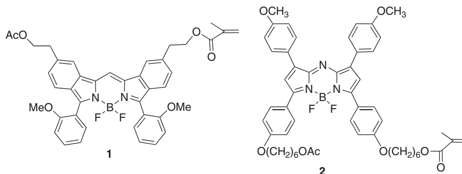
Scheme 1. Chemical structures of methacrylate-tethered red light-emitting dye 1 and NIR light-emitting dye 2 .
