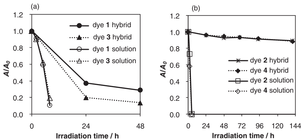
Figure 7. Photostability of solution and dye-incorporated PHEMA-silica hybrids prepared under microwave irradiation. (a) Red light-emitting dye 1 and 3 . (b) NIR light-emitting dye 2 and 4 . Concentrations of dye solutions were 1.0 \times 10^{-5} M. In the preparation of hybrids, the feed ratio of HEMA/MeTMOS was 1/2, and the molar ratio of HEMA/dye was 10000/1.
