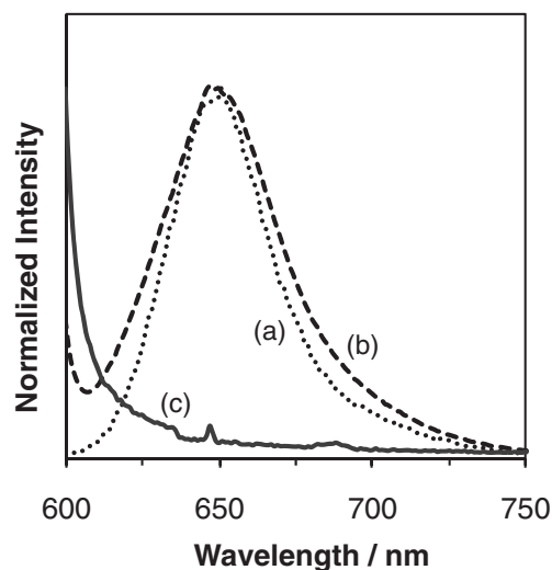
Figure 5. Photoluminescence spectra of (a) BODIPY dye 1 ( 1.0 \times 10^{-6} M THF solution), and dye 1-containing PHEMA-silica hybrids prepared under (b) microwave irradiation and (c) conventional heating. The feed ratio of HEMA/MeTMOS was 1/2. The molar ratio of HEMA/1 was 10000/1. Excitation wavelength: 590 nm.
