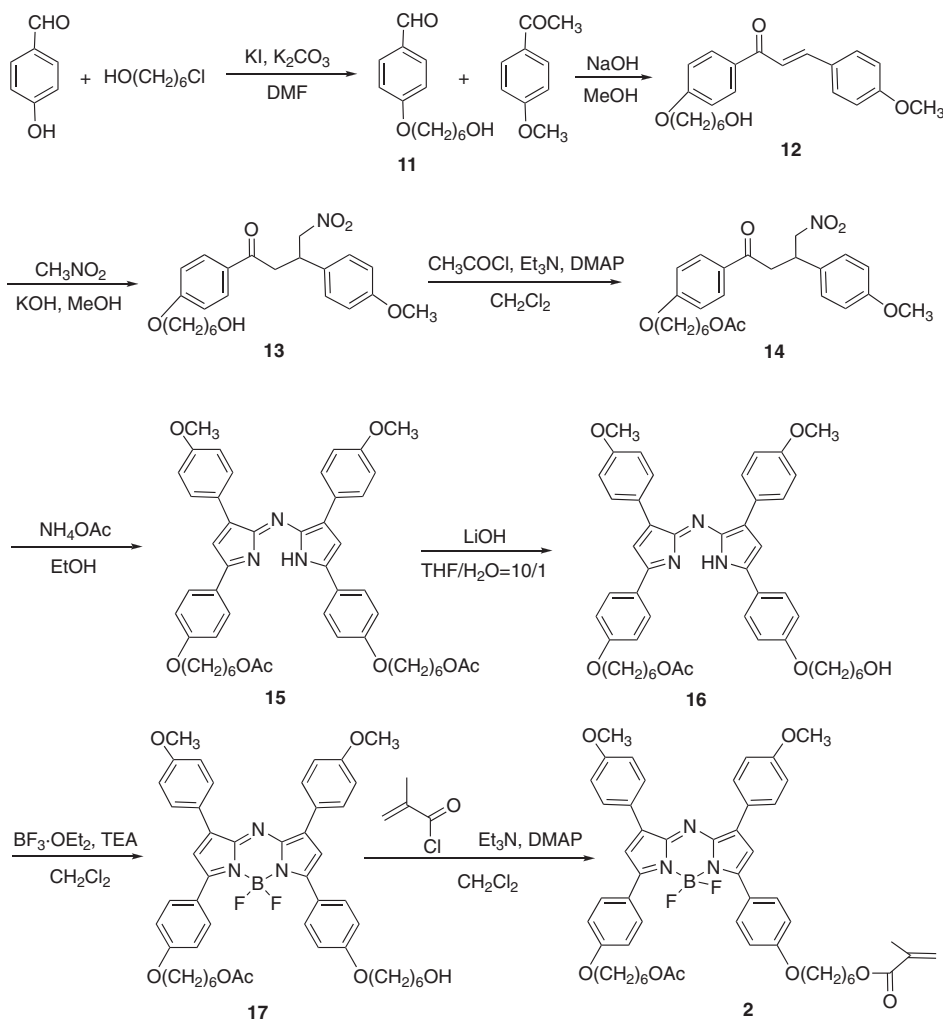
Scheme 3. Synthesis of methacrylate-tethered NIR light-emitting BODIPY dye 2.
