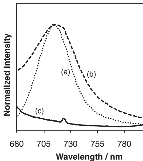
Figure 6. Photoluminescence spectra of (a) BODIPY dye 2 ( 1.0 \times 10^{-6} M THF solution), and dye 2-containing PHEMA-silica hybrids prepared under (b) microwave irradiation and (c) conventional heating. The feed ratio of HEMA/MeTMOS was 1/2. The molar ratio of HEMA/2 was 10000/1. Excitation wavelength: 660 nm.
